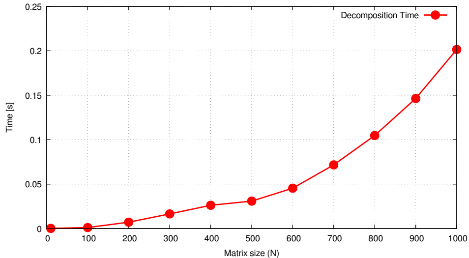
LU Decomposition Time Complexity ( O(N^3) )
