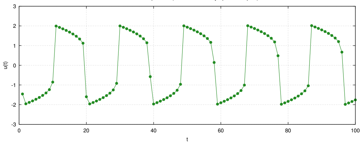
Ex 3: Fixed-Step Solver (Forced 100 Evenly Spaced Outputs)
