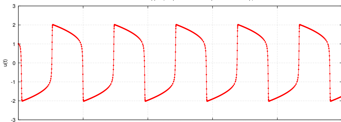
Ex 2: Low-Level Stepper (Outputs EVERY Adaptive Internal Step)
