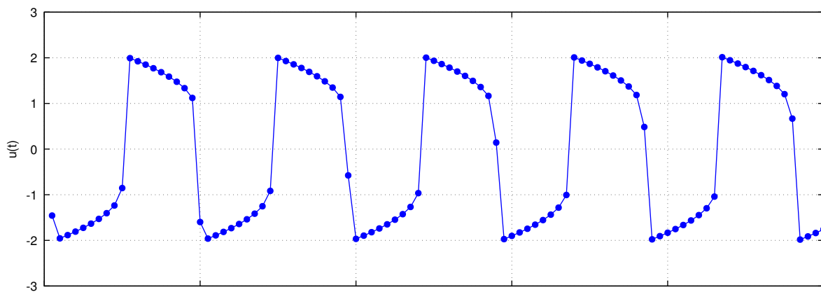
Ex 1: Adaptive Solver (Forced 100 Evenly Spaced Outputs)
