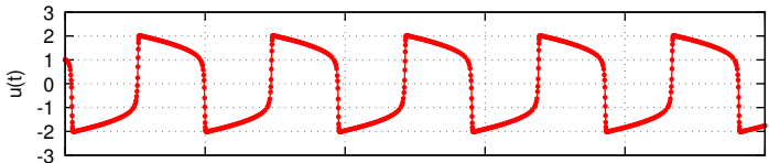
Ex 3: Fixed-Step Solver (Forced 100 Evenly Spaced Outputs)
