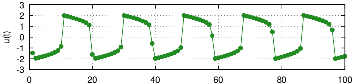
Ex 3: Fixed-Step Solver (Forced 100 Evenly Spaced Outputs)
