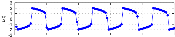
Ex 2: Low-Level Stepper (Outputs EVERY Adaptive Internal Step)
