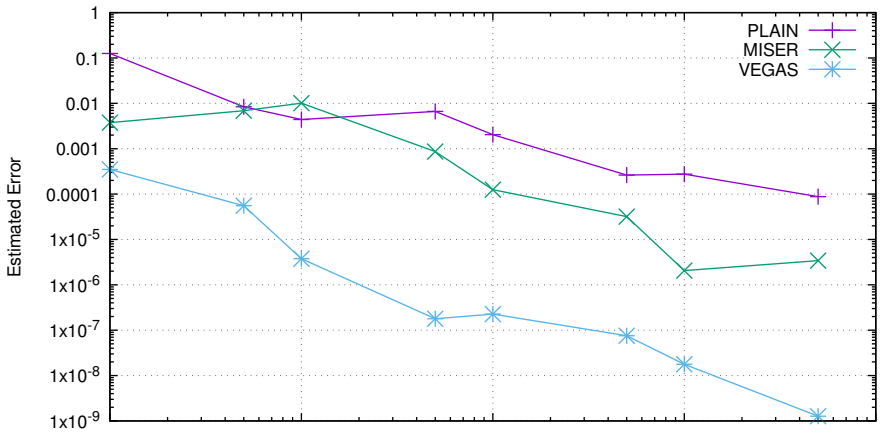
GSL Methods Error: f_1(x) = x^2 + x + 1
