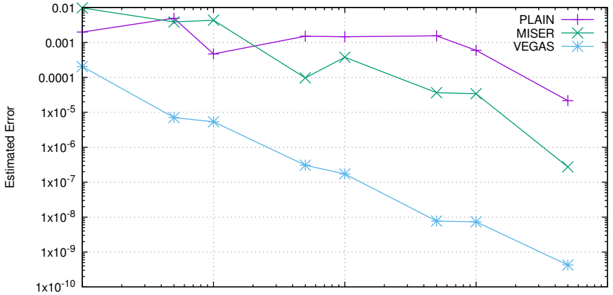
GSL Methods Error: f_2(x) = \sqrt{1-x^2}
