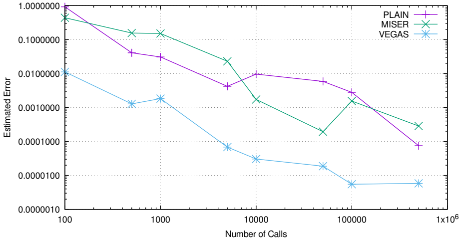
GSL Methods Error: f_3(x) = 1/\sqrt{x}
