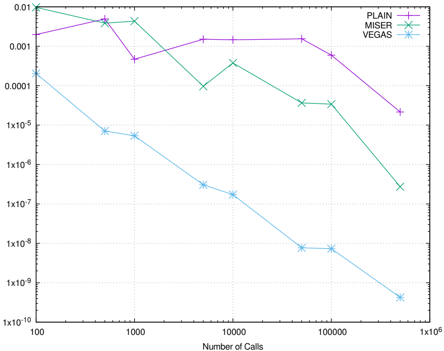
GSL Methods Error: f_2(x) = \sqrt{1-x^2}
