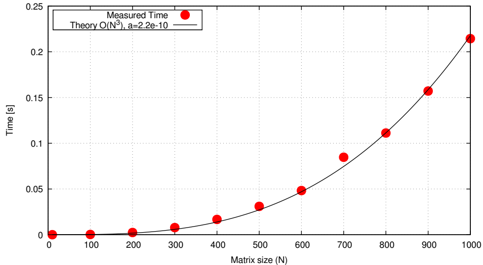
LU Decomposition: Measurement vs Theory O(N^3)
