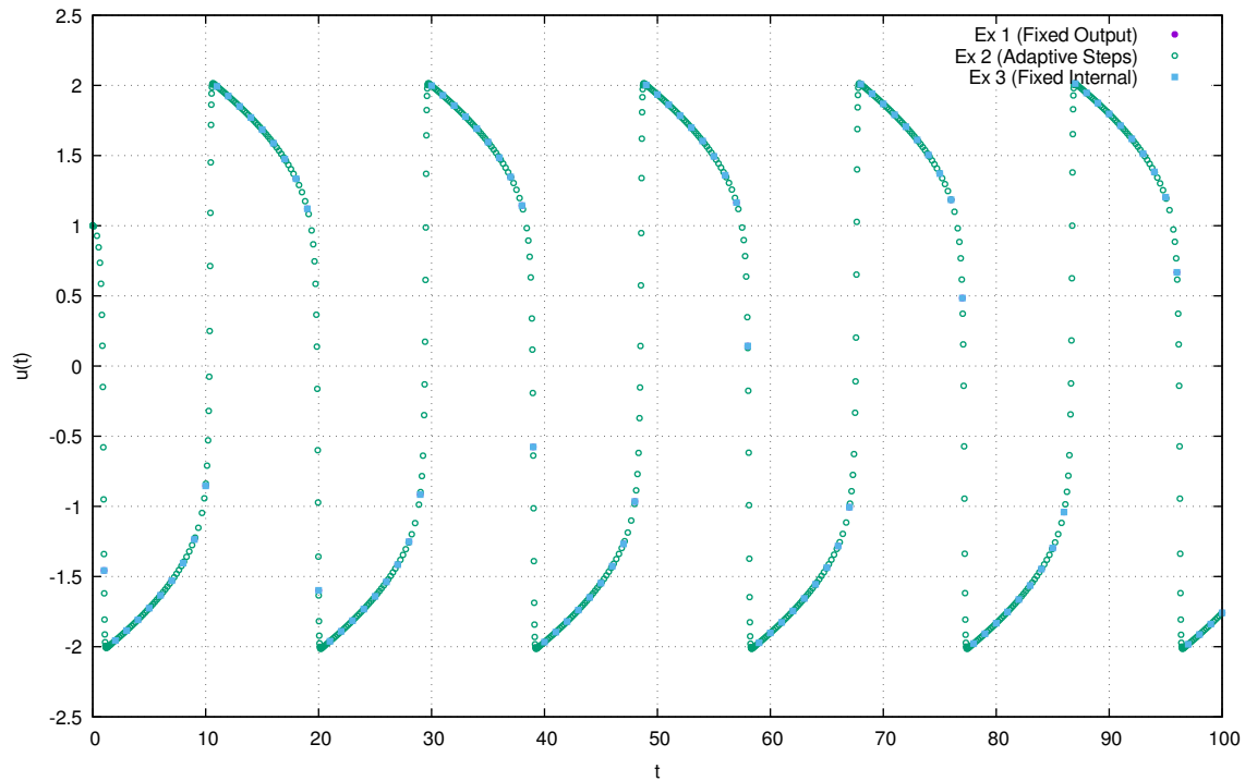
van der Pol Oscillator: u(t) vs t
