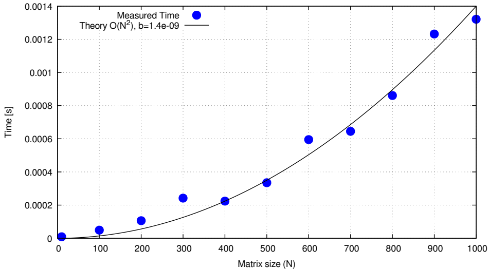
Solving: Measurement vs Theory O(N^2)
