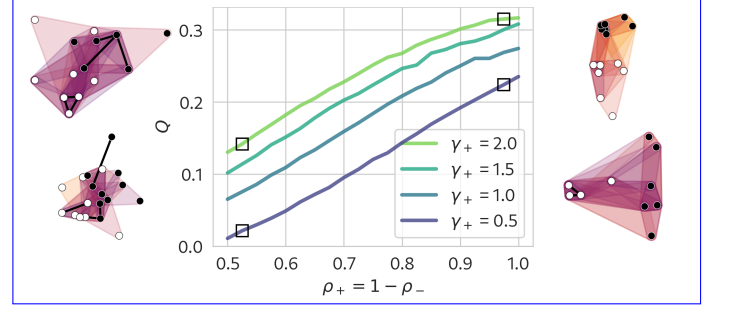
FIG. 1. Suite of model simulations illustrating the dependence of community structure, as measured by clique-projection modularity Q , on the CHILL parameters. The parameters \gamma_- = 0.5 , \eta_+ = 0.2 , and \eta_- = 0.1 are held fixed. Each line corresponds to a different value of \gamma_+ indicated by the legend. Along the horizontal axis, we vary \rho_+ and set \rho_- = 1 - \rho_+ . Each parameter combination is simulated 100 times for 1,000 timesteps. On either side of the plot, we show small hypergraphs sampled from parameter combinations indicated by the square markers for illustration.
