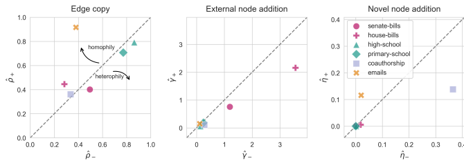
FIG. 4. Model parameters inferred via SEM for six empirical higher-order networks. The initial learning rate was \alpha^{(0)} = 0.01 , which exponentially decayed over iterations according to the exponent 0.001.
