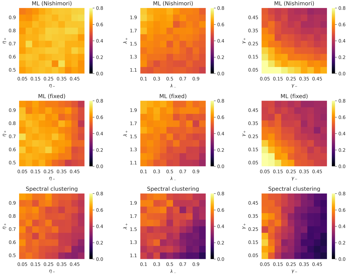
FIG. 5. Community detection results on synthetic data under the Nishimori condition [41] of exactly known parameters. Each pixel represents 200 independent hypergraphs generated from our model with 100 timesteps. The default parameters are (p_+, p_-, r_+, r_-, a_+, a_-) = (0.9, 0.1, 2.0, 0.3, 0.2, 0.1) ; in each panel, two of these parameters instead vary across the range shown on the axes. PC: This figure is probably a bit too bulky in comparison to the value it adds, consider ways to edit, compactify, or move part of it to supplementary.
