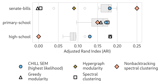
FIG. 6. Community detection results on three selected empirical datasets. Box plots describe the distribution of the ARI of CHILL SEM on the selected data set across 10 separate runs. The single label set achieving the highest likelihood under simulated annealing is highlighted. We compare these results with the ARI of the labels generated via several comparisons: hypergraph modularity [9] (only for senate-bills ), belief-propagation nonbacktracking spectral clustering [14], greedy dyadic modularity maximization [48], and dyadic Laplacian spectral clustering [46]; the latter two dyadic methods are denoted by hollow markers. Values for hypergraph modularity maximization and nonbacktracking spectral clustering are reported in [9] and [14], respectively.
