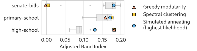
FIG. 6. Community detection results on three selected empirical datasets. Box plots describe the distribution of the ARI of simulated annealing on the selected data set across 10 separate runs. The single label set achieving the highest likelihood under simulated annealing is highlighted. We compare these results with the ARI of the labels generated via normalized spectral clustering and greedy modularity maximization.
