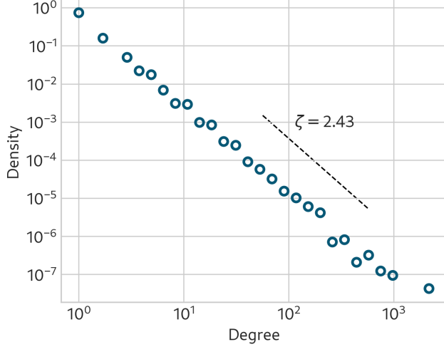
FIG. 5. Degree distribution from model simulation of 10^4 edges (points) and theoretical power law (line) with exponent given by Equation (2). The parameters in this experiment are \rho_+ = 0.7, \rho_- = 0.3, \gamma_+ = 0.5, \gamma_- = \eta_- 3, \eta_+ = 0.2, \eta_- = 0.1 .
