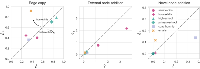
FIG. 4. Model parameters inferred via SEM for six empirical higher-order networks. PC: imo we need text and points to be a bit bigger here for legibility, not sure if we can do this as a single-column
