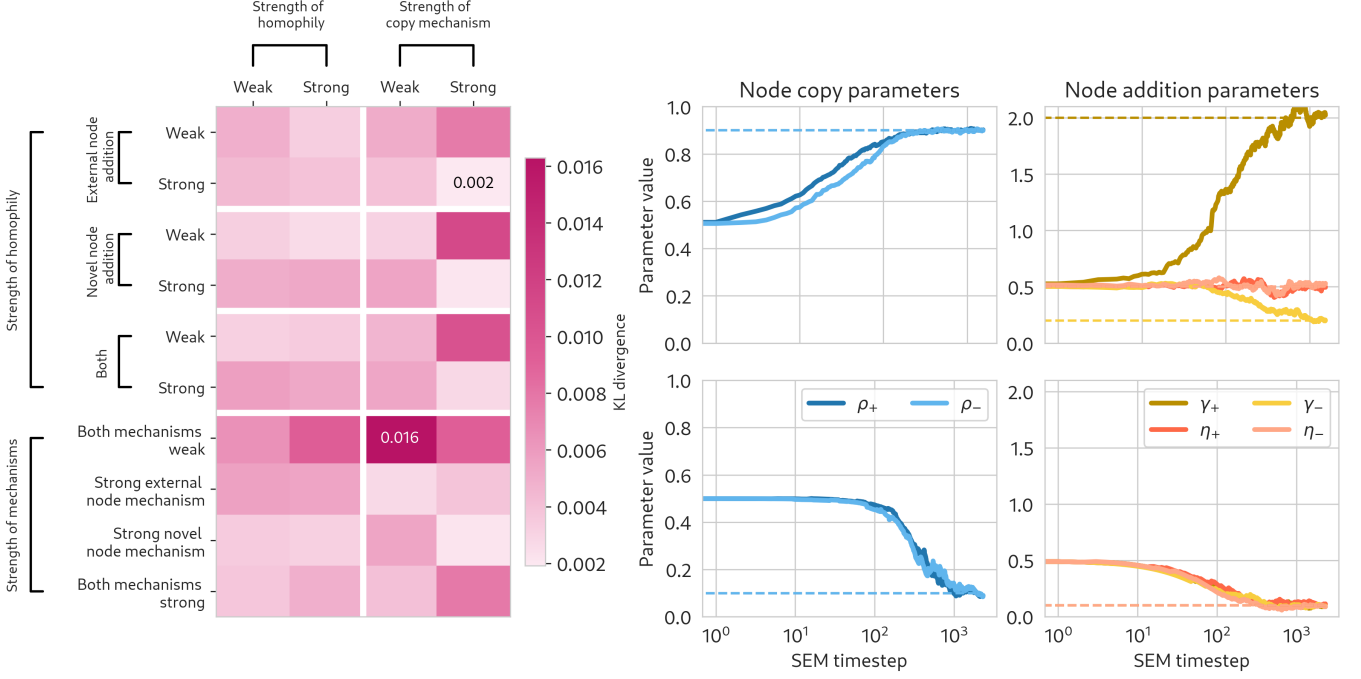
FIG. 3. Performance of SEM on synthetic hypergraphs. Each entry in the heatmap corresponds to a set of parameters \theta , specified in Appendix G. For each set of parameters, five independent hypergraphs are generated according to the model and SEM is performed independently on each. The Kullback-Leibler (KL) divergence between the true and estimated parameters is then computed for each of the five estimated parameter vectors \hat{\theta}_i generated by SEM. The color of an entry in the heatmap represents the mean KL divergence over the five simulations for that set of parameters. Details on the parameters used in these simulations can be found in Section G, Table II.
