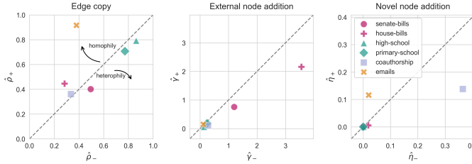
FIG. 5. Model parameters inferred via SEM for six empirical higher-order networks. PC: imo we need text and points to be a bit bigger here for legibility, not sure if we can do this as a single-column
