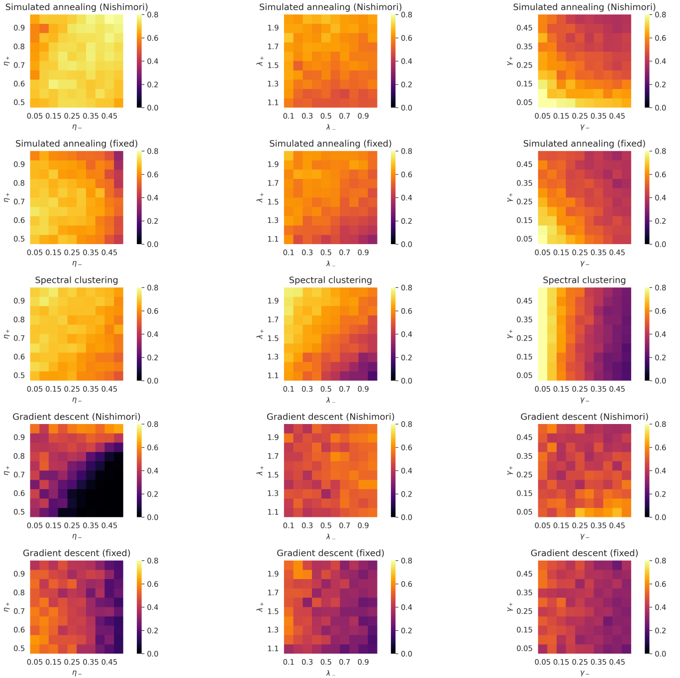
FIG. 4. Community detection results on synthetic data under the Nishimori condition [40] of exactly known parameters. Each pixel represents 100 independent hypergraphs generated from our model with 100 timesteps. The default parameters are (p_+, p_-, r_+, r_-, a_+, a_-) = (0.9, 0.1, 2.0, 0.3, 0.2, 0.1) ; in each panel, two of these parameters instead vary across the range shown on the axes. PC: This figure is probably a bit too bulky in comparison to the value it adds, consider ways to edit, compactify, or move part of it to supplementary.
