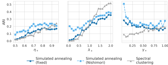
FIG. 5. Comparison of community detection methods on synthetic data. We compare our simulated annealing algorithm under the Nishimori condition and with a fixed parameter vector \theta' = (0.9, 0.1, 0.2, 0.1, 2.0, 0.3) against a baseline of Laplacian spectral clustering on the weighted clique projection of the hypergraph. The “default” parameter vector used is \theta = (\rho_+, \rho_-, \gamma_+, \gamma_-, \eta_+, \eta_-) = (0.8, 0.15, 0.8, 0.5, 0.7, 0.2) . In each of the three panels, a single one of these parameters is varied while the others are held fixed at their default values. Each point gives the mean ARI over 500 independent model simulations, each of which were simulated for 200 timesteps.
