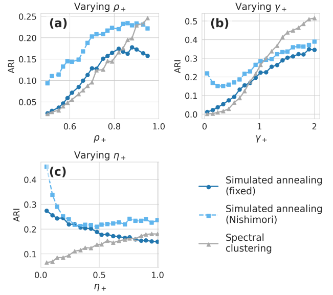
FIG. 5. Comparison of community detection methods on synthetic data. We compare our simulated annealing algorithm under the Nishimori condition and with a fixed parameter vector \theta' = (0.9, 0.1, 0.2, 0.1, 2.0, 0.3) against a baseline of Laplacian spectral clustering on the weighted clique projection of the hypergraph. The “default” parameter vector used in synthetic hypergraph generation is \theta = (\rho_+, \rho_-, \gamma_+, \gamma_-, \eta_+, \eta_-) = (0.8, 0.15, 0.8, 0.5, 0.7, 0.2) . In each of the three panels (a-c), a single one of these parameters is varied while the others are held fixed at their default values. Each point gives the mean ARI over 500 independent model simulations, each of which was simulated for 200 timesteps.
