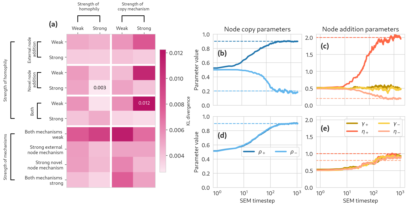
FIG. 3. Performance of SEM on synthetic hypergraphs. Each pixel in the heatmap (panel (a)) corresponds to a set of parameters \theta , which can be found in Appendix C. For each set of parameters, 20 independent hypergraphs are simulated under the CHILL model for 2,000 simulation steps. We then perform SEM on each. Finally, we compute the Kullback-Leibler (KL) divergence of the estimated parameters from the true ones (eq. (6)) and average the results to obtain a value in a pixel. The parameter estimates over iterations of SEM are plotted for the underlying parameters which produced the lowest mean KL divergence (copy parameters in panel (b) and addition parameters in panel (c)), and similarly for the parameters that produced the highest mean KL divergence in panels (d) and (e).
