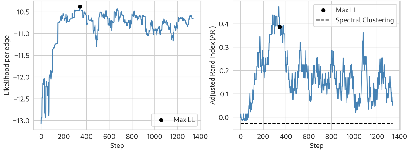
FIG. 9. Illustrative run of simulated annealing for community detection in a hypergraph generated from our model. The dashed line on the right shows the ARI achieved by Laplacian spectral clustering applied to the weighted dyadic graph projection. Solid point gives the highest likelihood and corresponding ARI achieved by simulated annealing over the course of the run.
