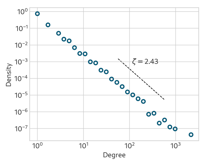
FIG. 7. Degree distribution from model simulation of 10^4 edges (points) and theoretical power law (line) with exponent given by Equation (2). The parameters in this experiment are \rho_+ = 0.7, \rho_- = 0.3, \gamma_+ = 0.5, \gamma_- = \eta_-3, \eta_+ = 0.2, \eta_- = 0.1 .
