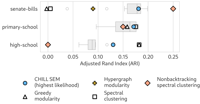
FIG. 6. Community detection results on three selected empirical data sets. Box plots describe the distribution of the ARI of CHILL simulated annealing on the selected data set across 10 separate runs.
