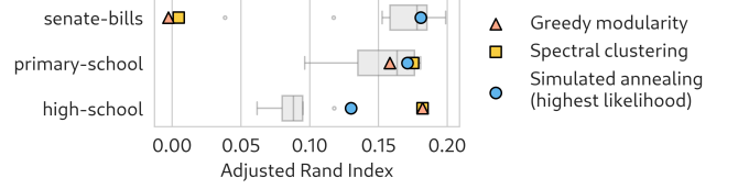
FIG. 5. Community detection results on empirical datasets.
