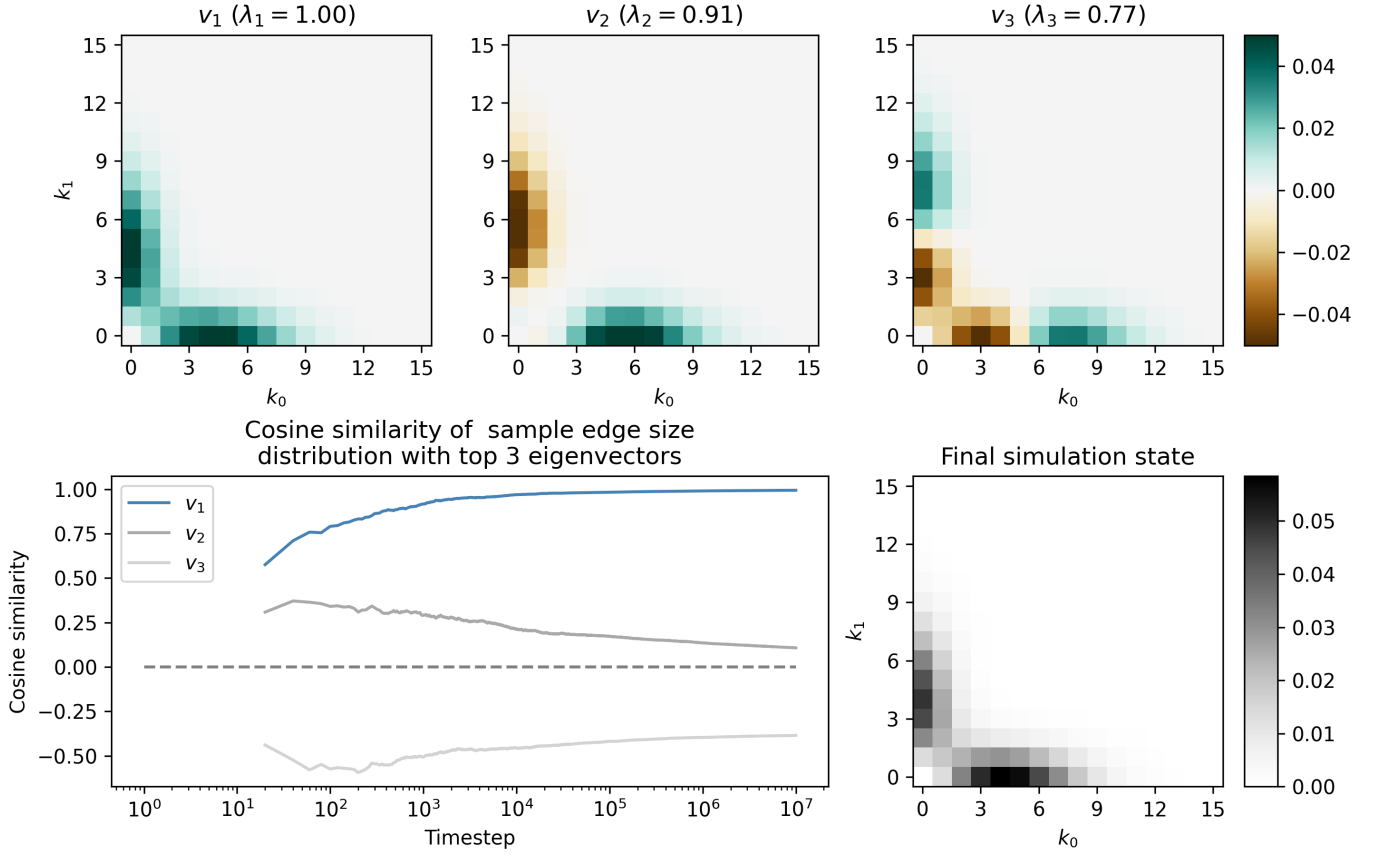
FIG. 2. Dynamics! Top shows the three leading eigenvectors of the distribution p(k_0, k_1) . Bottom left gives the cosine similarity (normalized projection) between one run of simulation dynamics and these eigenvectors. Bottom right gives the final simulation state. PC: Need to check these projections, looks a bit strange. Can run 10^7 steps in two minutes on laptop.
