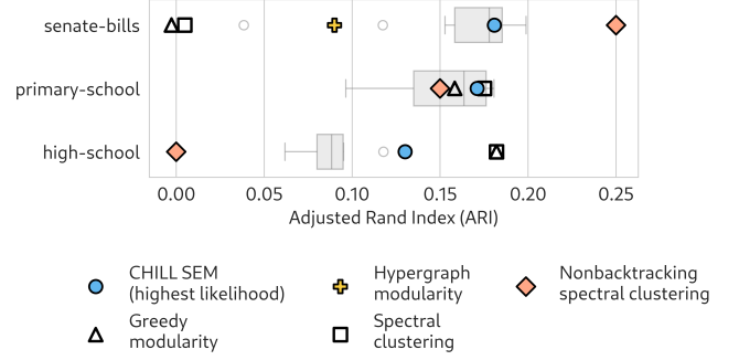
FIG. 6. Community detection results on three selected empirical data sets. Box plots describe the distribution of the ARI of CHILL simulated annealing on the selected data set across 10 separate runs.
