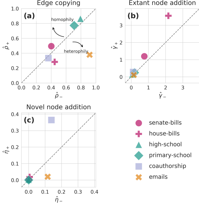
FIG. 4. Model parameters inferred via SEM for six empirical higher-order networks. The line of equality is shown as a guide for the eye.
