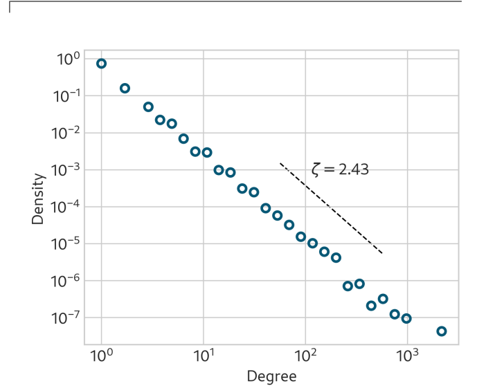
FIG. 7. Degree distribution from model simulation of 10^4 edges (points) and theoretical power law (line) with exponent given by Equation (2). The parameters in this experiment are \rho_+ = 0.7, \rho_- = 0.3, \gamma_+ = 0.5, \gamma_- = \eta_- 3, \eta_+ = 0.2, \eta_- = 0.1 .
