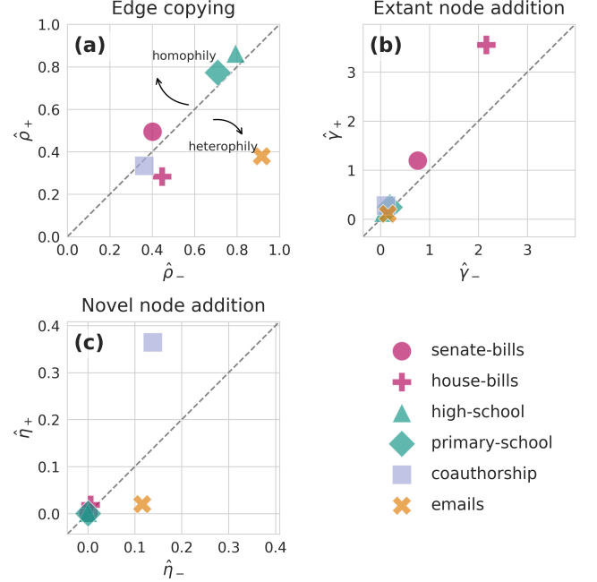
FIG. 4. Model parameters inferred via SEM for six empirical higher-order networks. The line of equality is shown as a guide for the eye.
