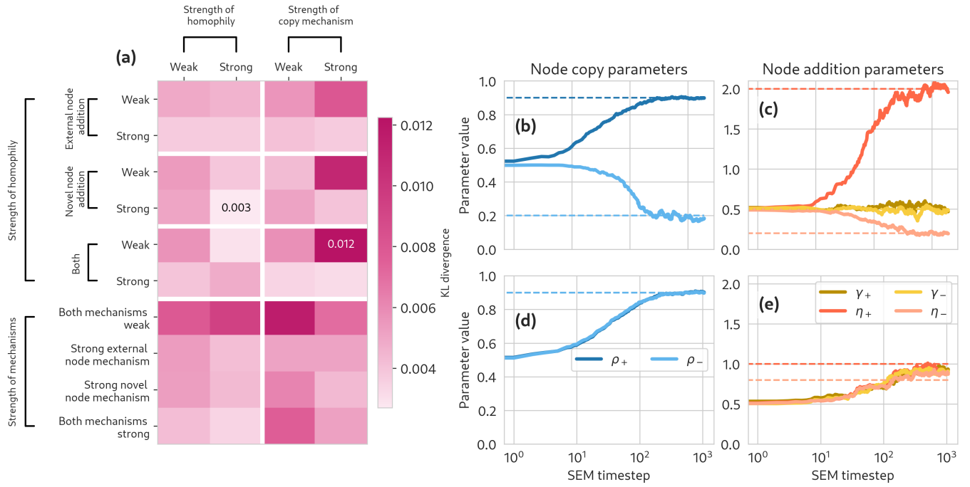
FIG. 3. Performance of SEM on synthetic hypergraphs. Each entry in the heatmap (panel (a)) corresponds to a set of parameters \theta , which can be found in Appendix C. For each set of parameters, 20 independent hypergraphs are simulated under the CHILL model for 2,000 simulation steps. We then perform SEM on each. We then compute the Kullback-Leibler (KL) divergence of the estimated parameters from the true ones (eq. (6)) and average the results to obtain a value in a pixel. The parameter estimates over iterations of SEM are plotted for the underlying parameters which produced the lowest mean KL divergence (copy parameters in panel (b) and addition parameters in panel (c)), and similarly for the parameters that produced the highest mean KL divergence in panels (d) and (e).
