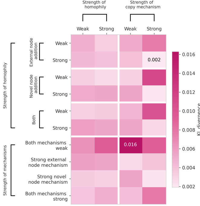
FIG. 4. Performance of SEM on synthetic hypergraphs. Each entry in the heatmap corresponds to a set of parameters \theta , specified in Appendix ?? . For each set of parameters, five independent hypergraphs are generated according to the model and SEM is performed independently on each. The Kullback-Leibler (KL) divergence between the true and estimated parameters is then computed for each of the five estimated parameter vectors \hat{\theta}_i generated by SEM. The color of an entry in the heatmap represents the mean KL divergence over the five simulations for that set of parameters.
