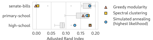
FIG. 5. Community detection results on three selected empirical datasets. Box plots describe the distribution of the ARI of simulated annealing on the selected data set across 10 separate runs. The single label set achieving the highest likelihood under simulated annealing is highlighted. We compare these results with the ARI of the labels generated via normalized spectral clustering and greedy modularity maximization.
