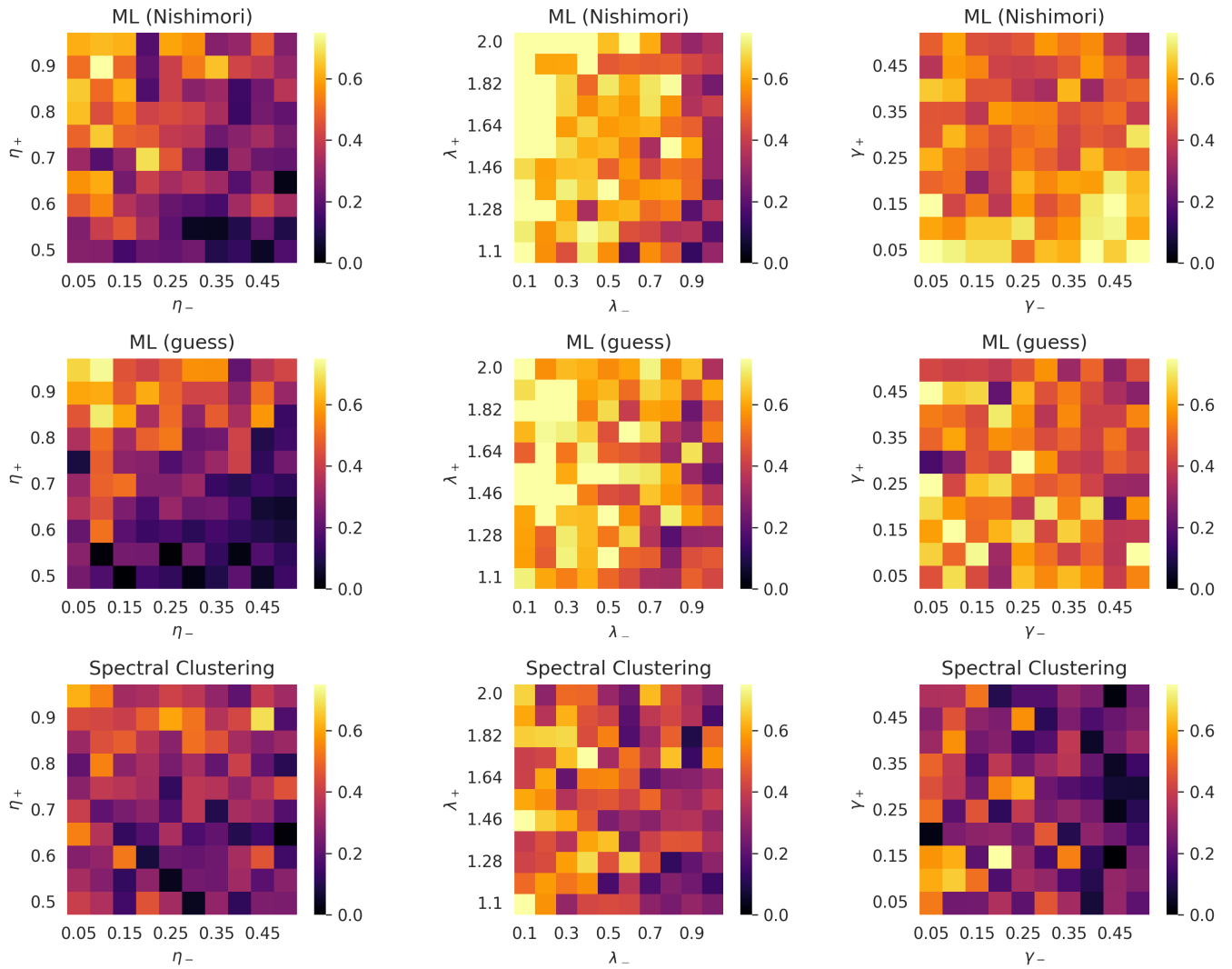
FIG. 4. Community detection results on synthetic data under the Nishimori condition [35] of exactly known parameters.
