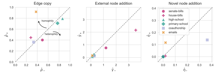
FIG. 5. Model parameters inferred via SEM for six empirical higher-order networks.
