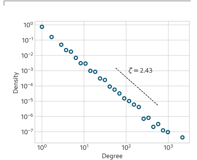
FIG. 5. Degree distribution from model simulation of 10^4 edges (points) and theoretical power law (line) with exponent given by Equation (2). The parameters in this experiment are \rho_+ = 0.7, \rho_- = 0.3, \gamma_+ = 0.5, \gamma_- = \eta_-3, \eta_+ = 0.2, \eta_- = 0.1 .
