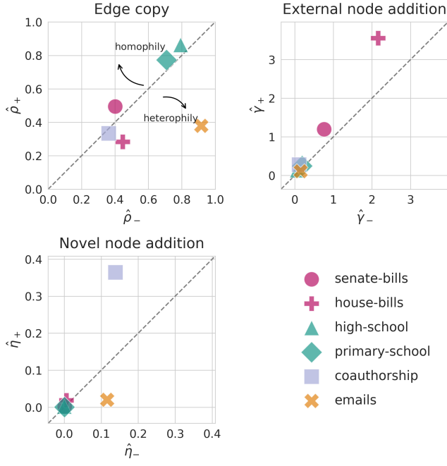
FIG. 4. Model parameters inferred via SEM for six empirical higher-order networks. PC: imo we need text and points to be a bit bigger here for legibility, not sure if we can do this as a single-column
