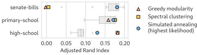
FIG. 6. Community detection results on three selected empirical datasets. Box plots describe the distribution of the ARI of simulated annealing on the selected data set across 10 separate runs. The single label set achieving the highest likelihood under simulated annealing is highlighted. We compare these results with the ARI of the labels generated via normalized spectral clustering and greedy modularity maximization.
