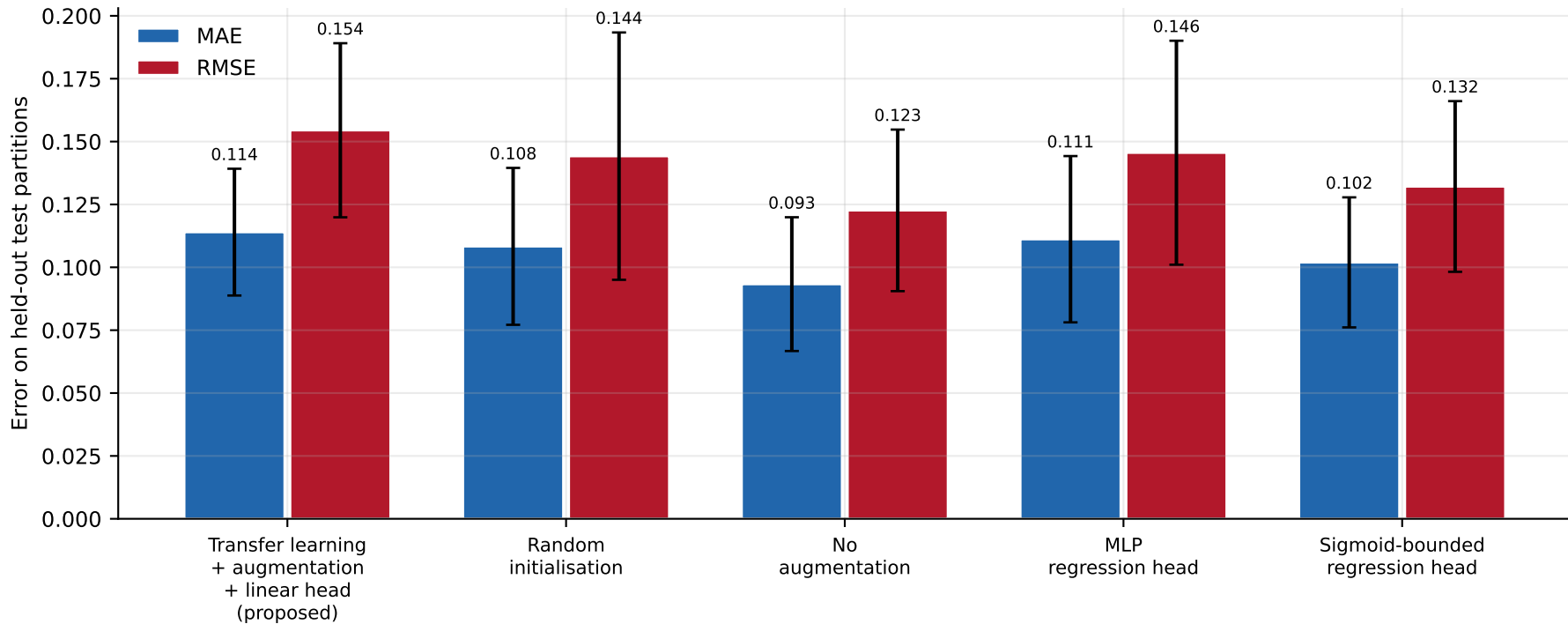
Ablation study: contribution of transfer learning, augmentation and regression-head design (mean \pm SD over six source-disjoint folds)
