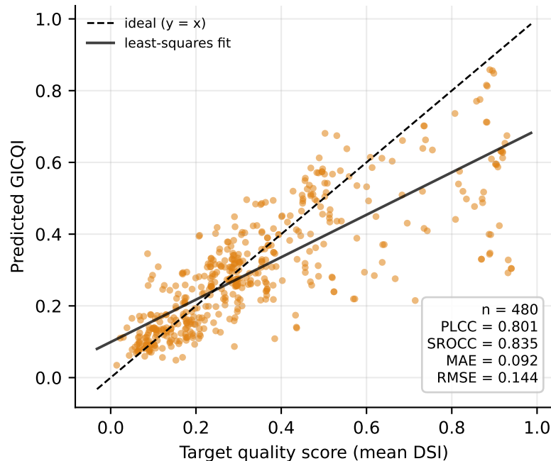
(b) Validation partition
