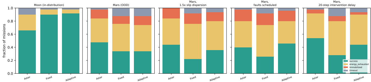
Figure 2: How missions ended. Descriptively, the adaptive planner ends fewer missions in energy exhaustion than the fixed planner in every condition. This was not a pre-specified test.
