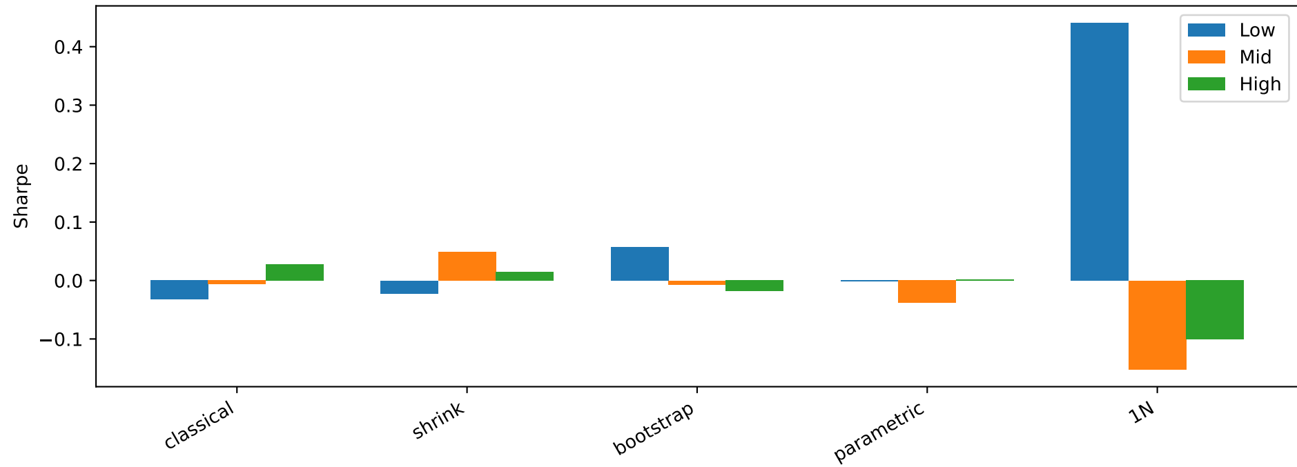
Regime-specific Sharpe by Method
