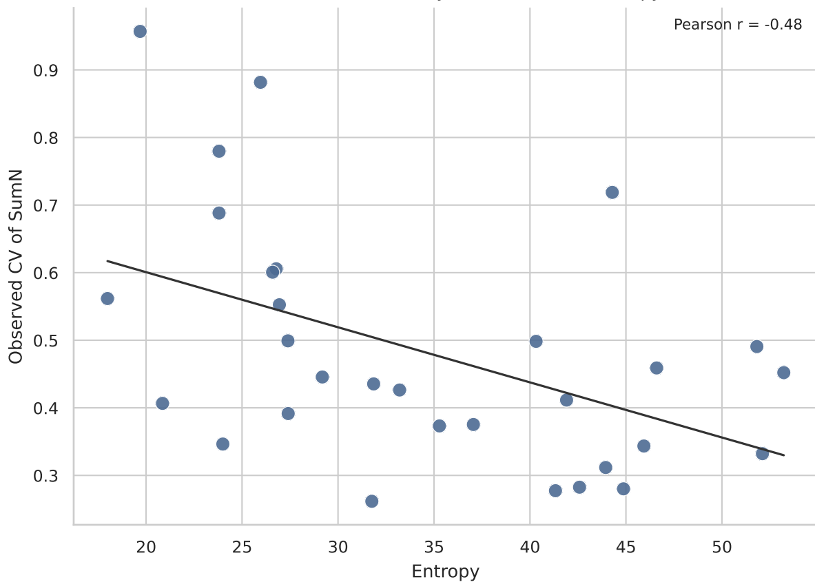
Pooled control variability versus network entropy
