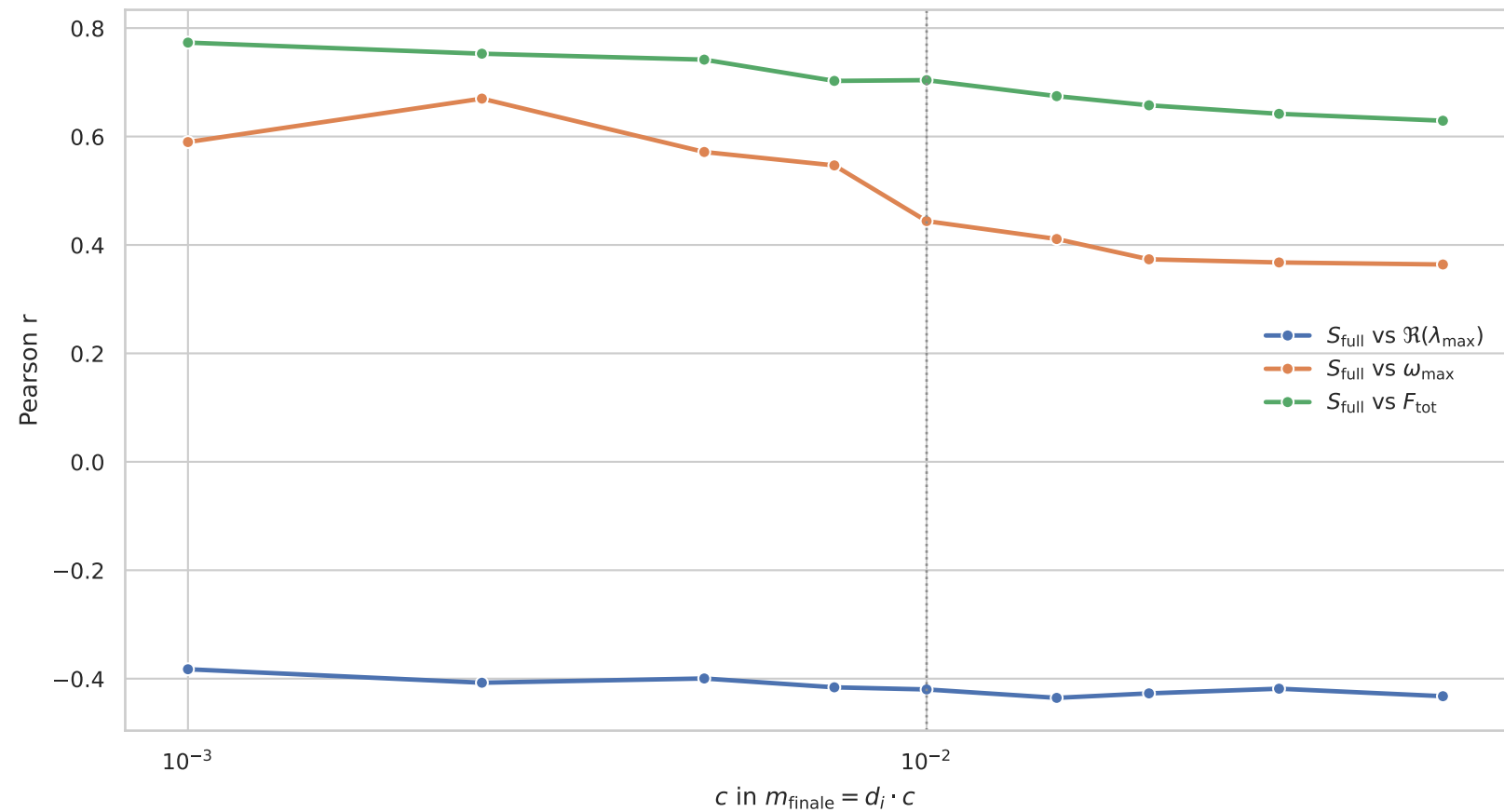
Trajectories of S_{\text{full}} relationships across the m_{\text{finale}} grid
