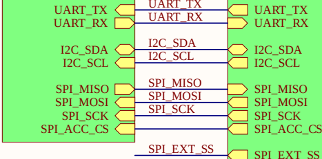
EXT_Devices2 ExtDevices2_sheet.SchDoc
