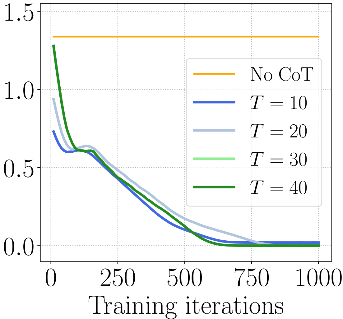
Test loss
