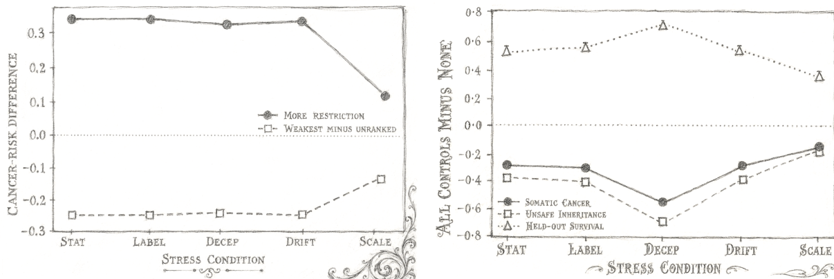
Figure 3: Frozen confirmatory results across stationary positive-only, label-free, strategic-deception, continual-representation-change, and scaled conditions. Left panel shows cancer-risk effects of added restriction and weakest-correct selection. Right panel shows combined-control effects. Error bars are 95% bootstrap intervals over worlds.
