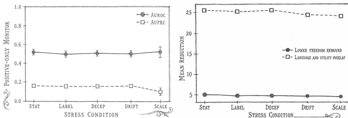
Figure 4: Limits and stack effects in frozen confirmatory runs. Positive-only monitor performance remained near chance. Stronger lower restriction reduced lower freedom, induced higher-layer language size, and higher-layer utility in every condition. The latter two lines overlap.
