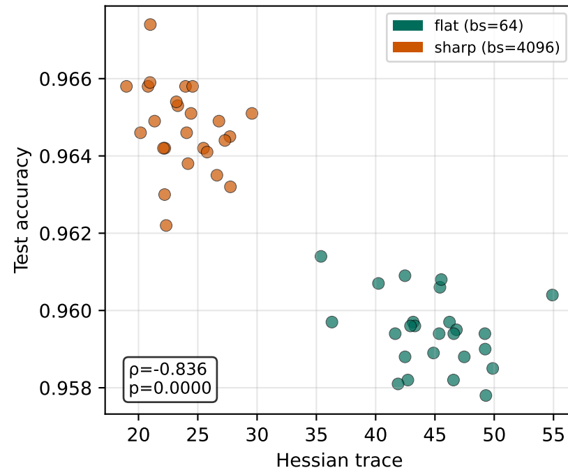
(a) Sharpness
