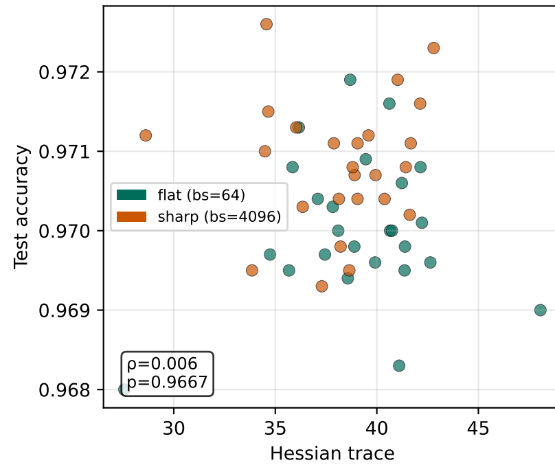
(a) Sharpness
