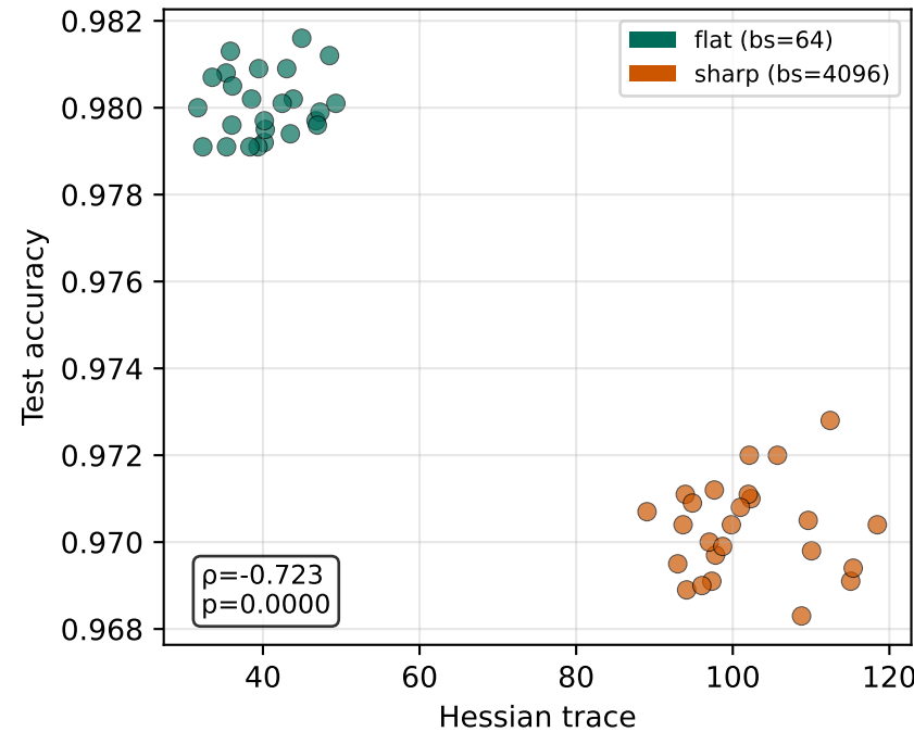
(a) Sharpness
