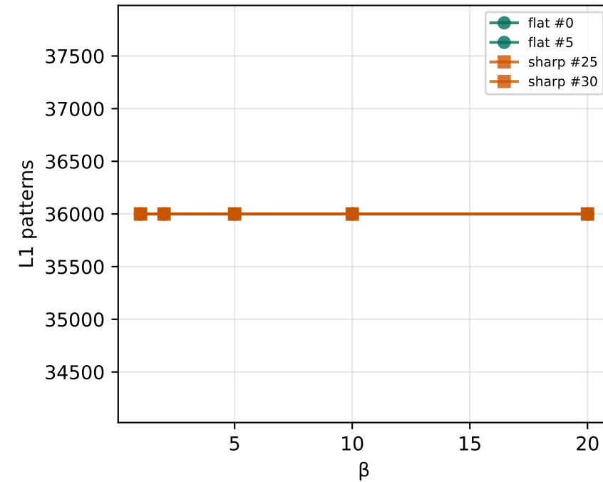
(c) Activation patterns invariant
