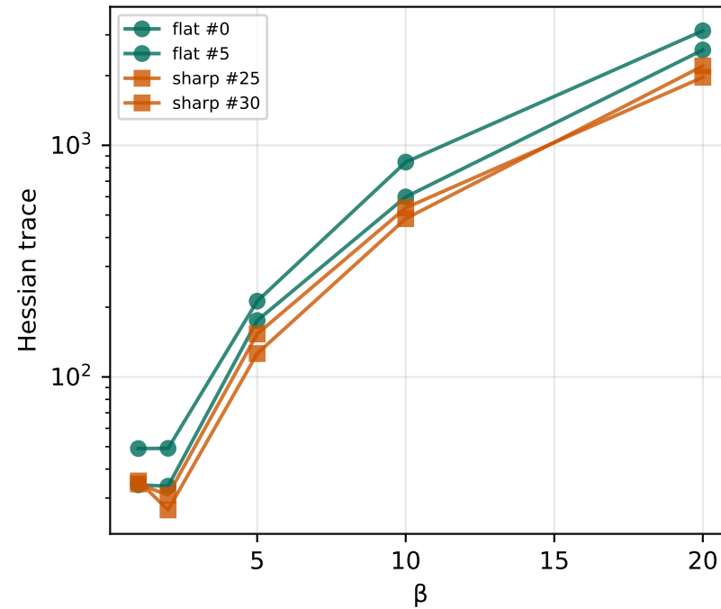
(a) Sharpness changes
