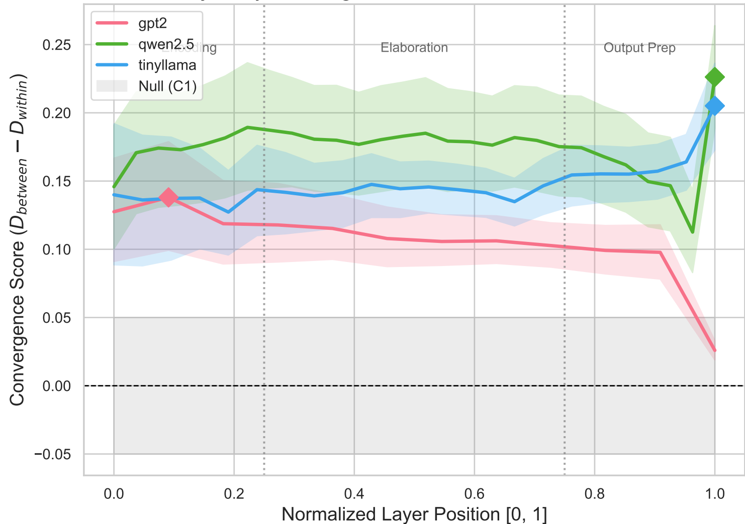
Trajectory Convergence Index Across Architectures
