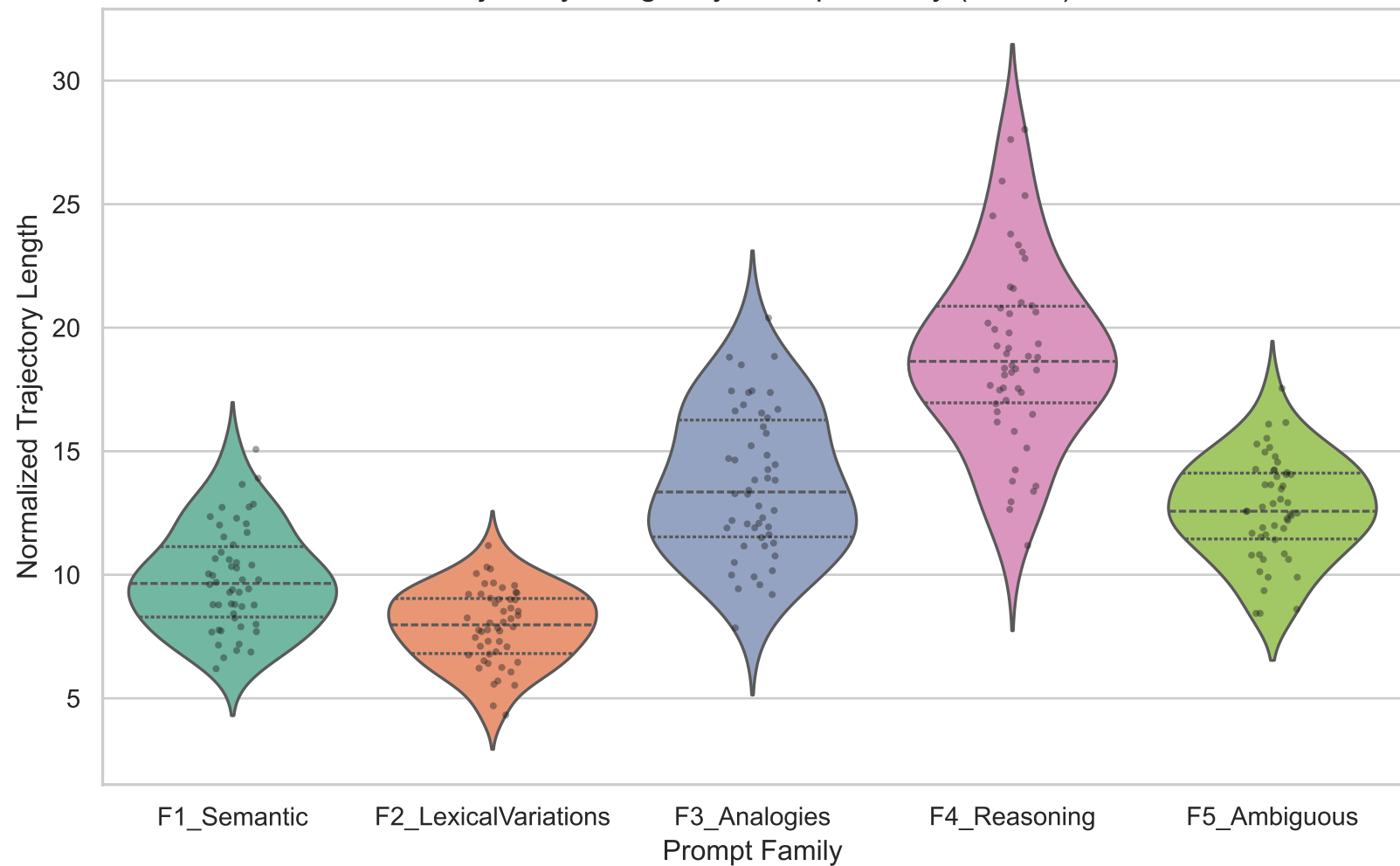
Trajectory Length by Prompt Family (F1–F5)
