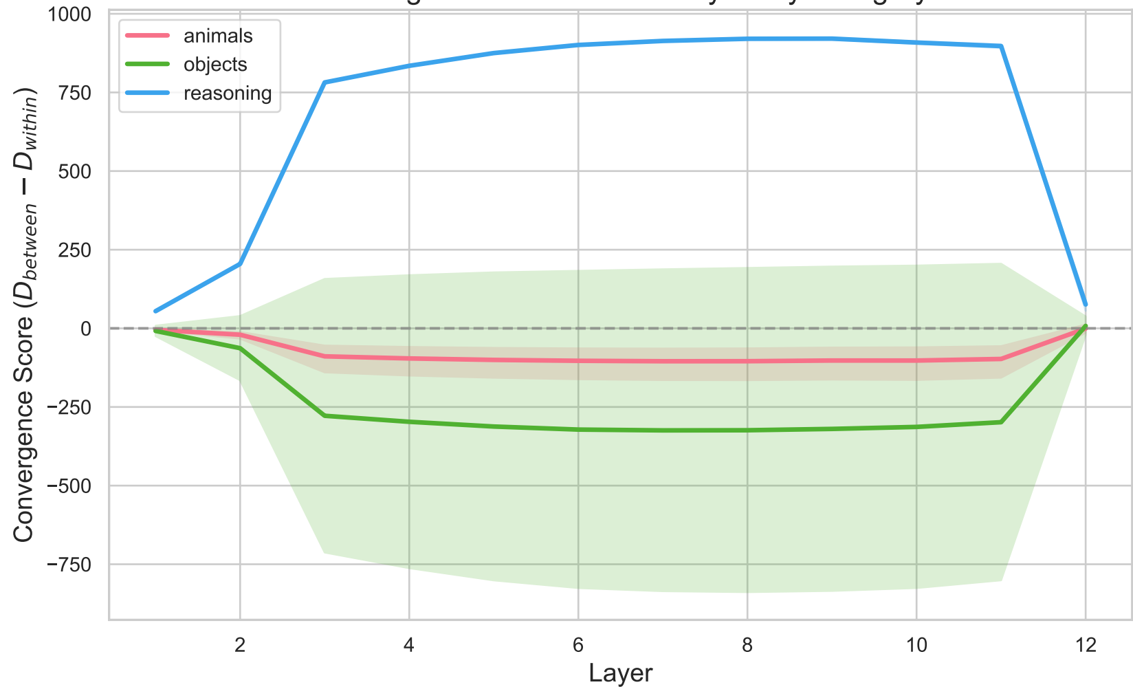
Convergence Score Across Layers by Category
