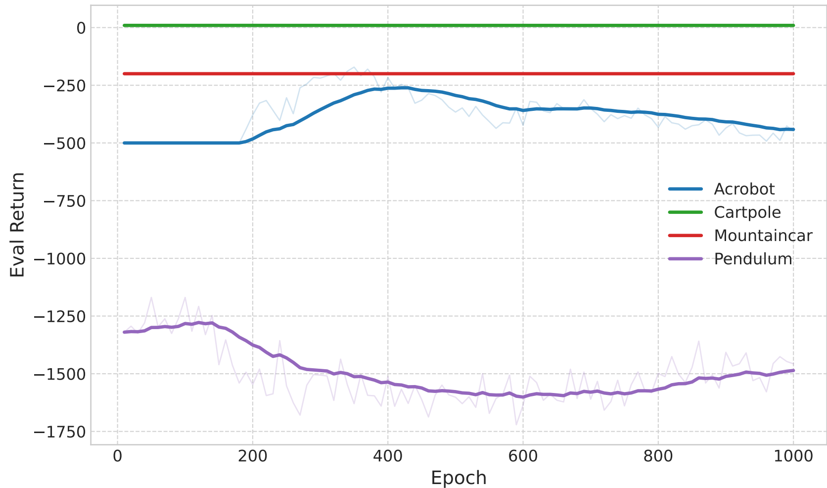
Decision Transformer Performance
