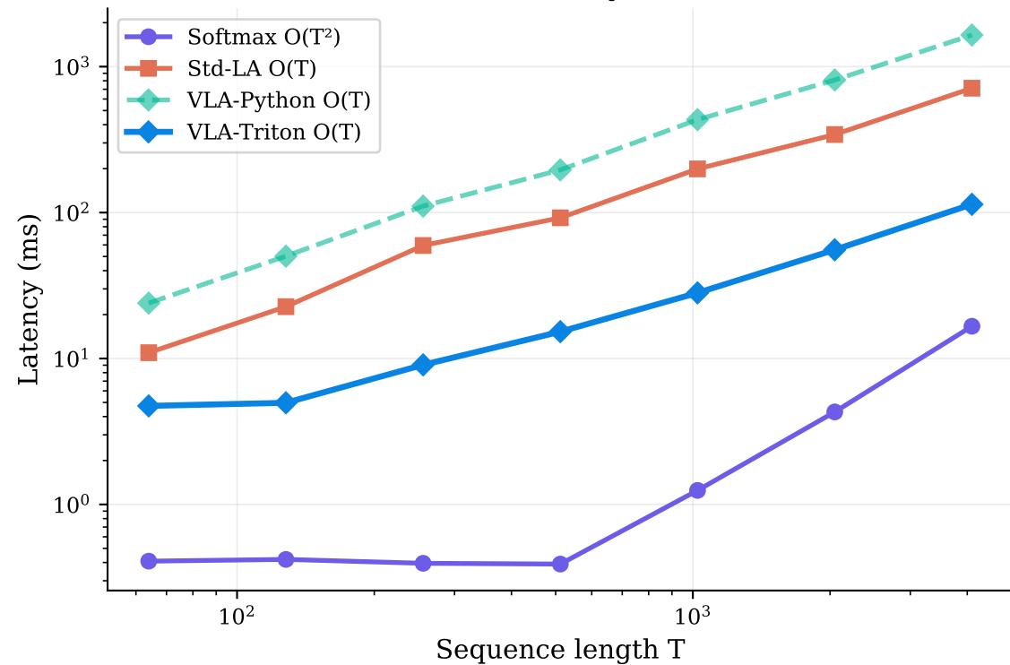
Forward Pass Latency (d=64, B=4)
