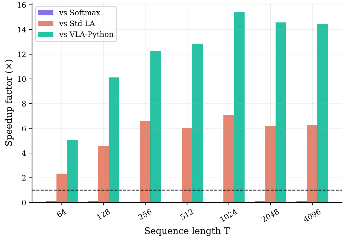
VLA-Triton Speedup
