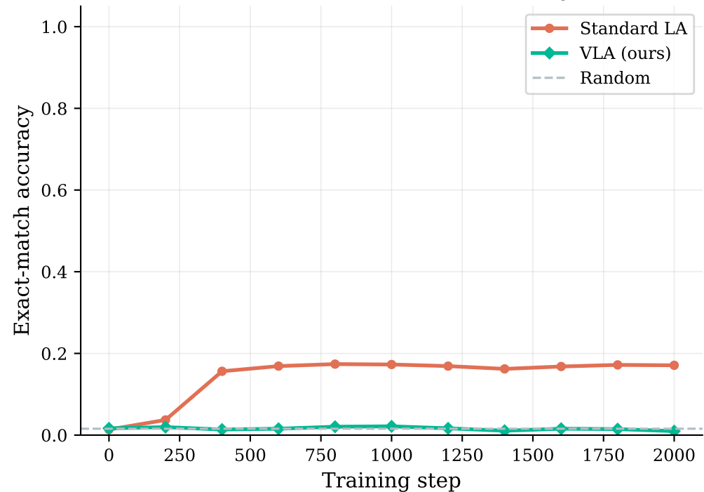
(b) MQAR Retrieval Accuracy
