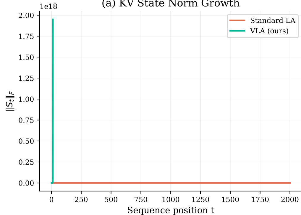
(a) KV State Norm Growth
