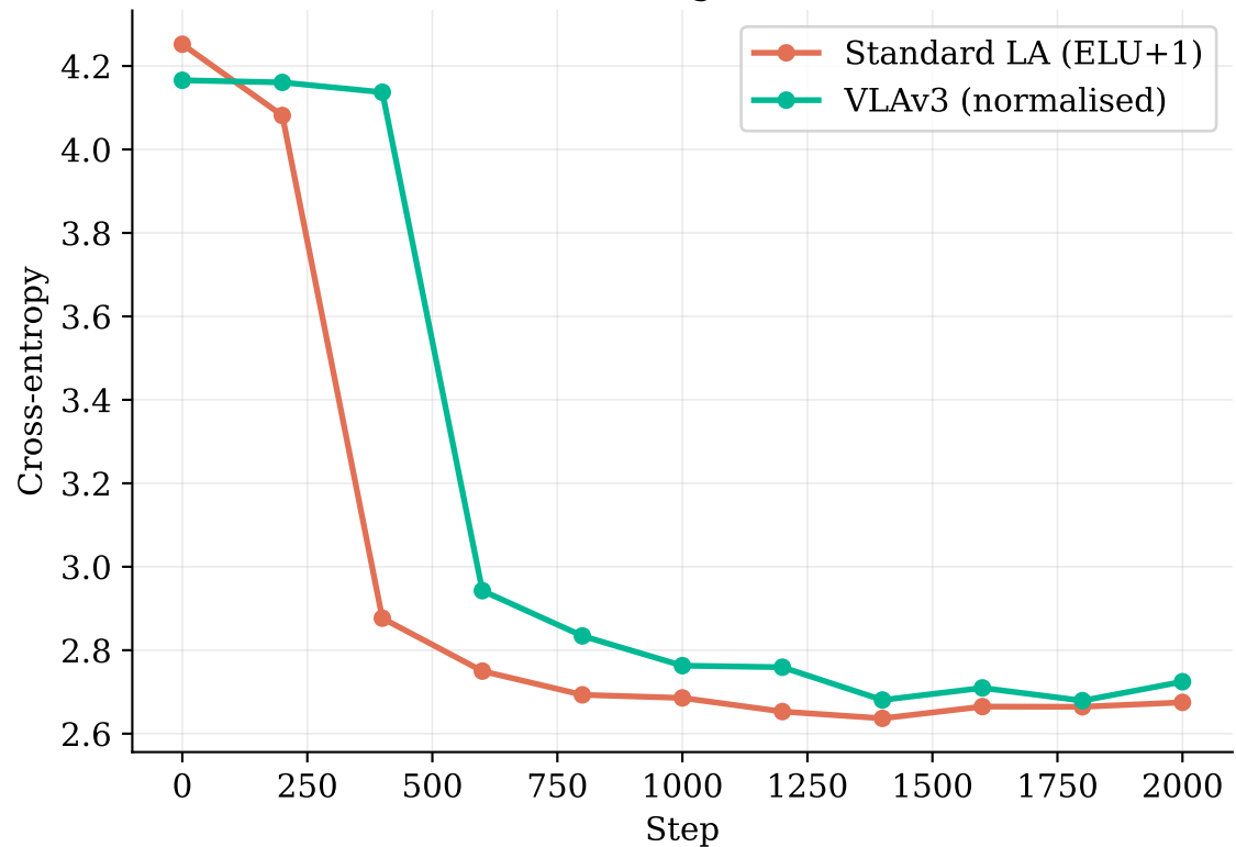
Training Loss
