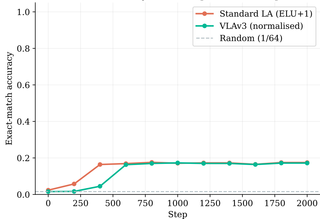
MQAR Accuracy (d=64, 8 pairs, 2000 steps)
