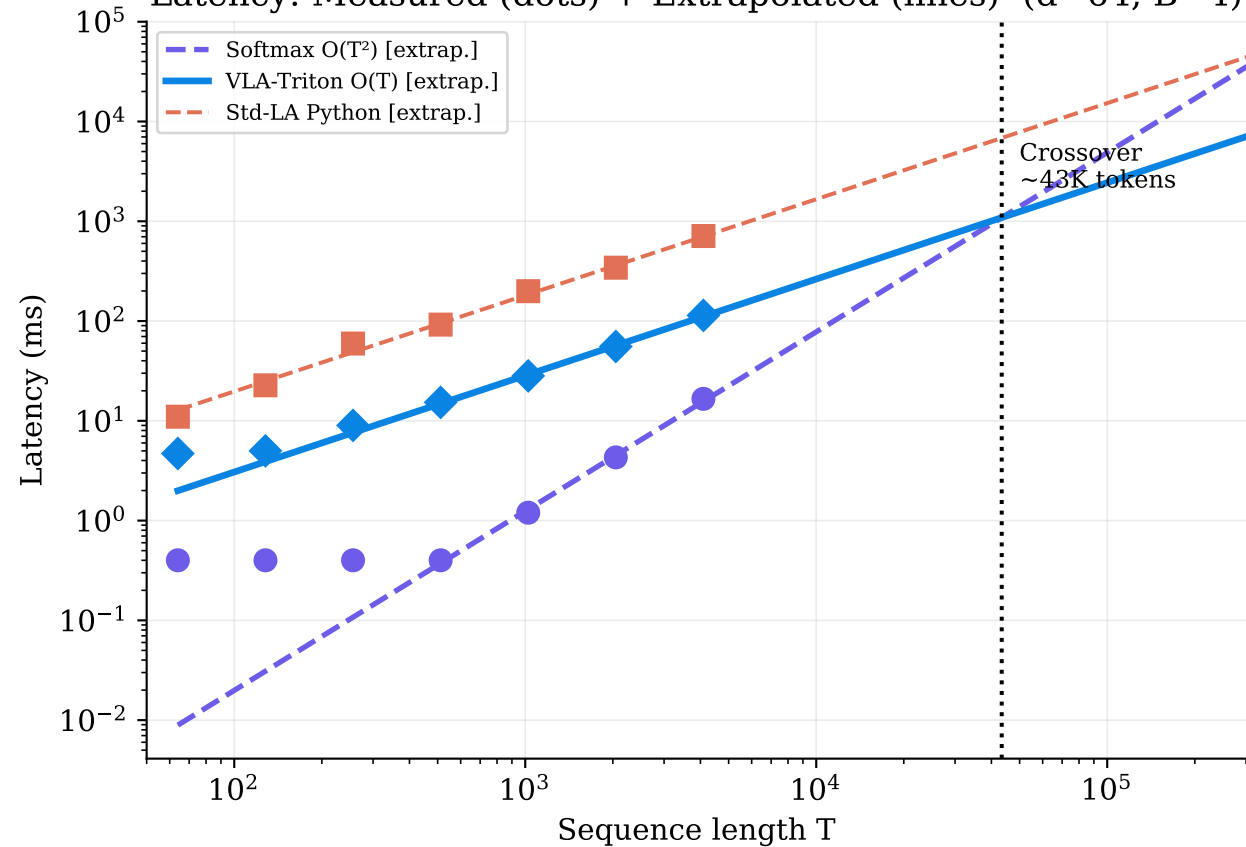
Latency: Measured (dots) + Extrapolated (lines) (d=64, B=4)
