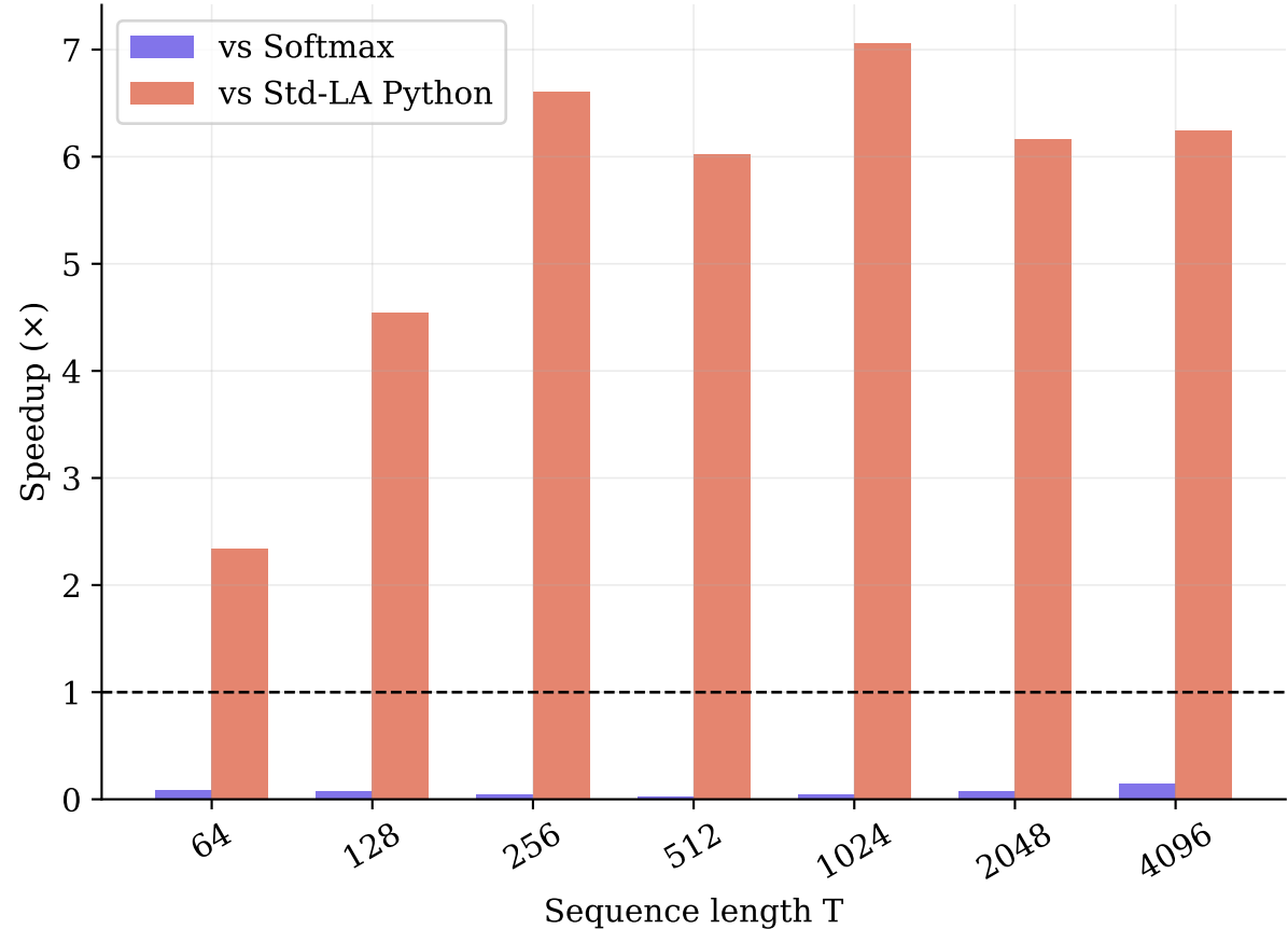
VLA-Triton Speedup Factor
